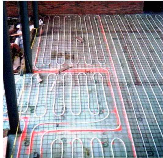
Hydronic Floor Slab Heat Tubing
