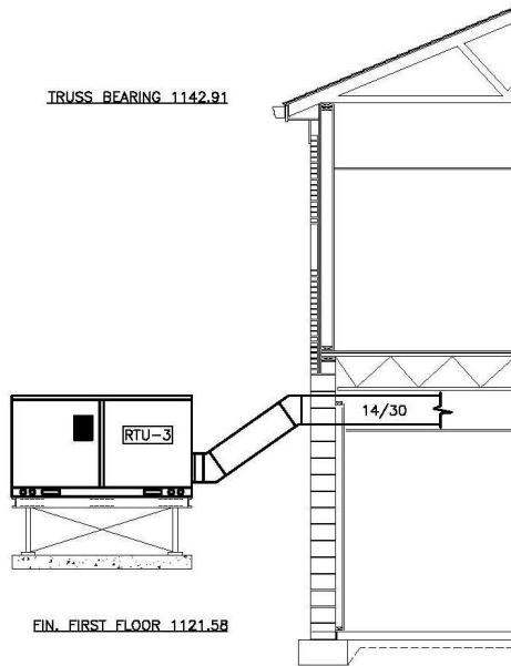
RTU-3 SUPPORT ELEVATION
